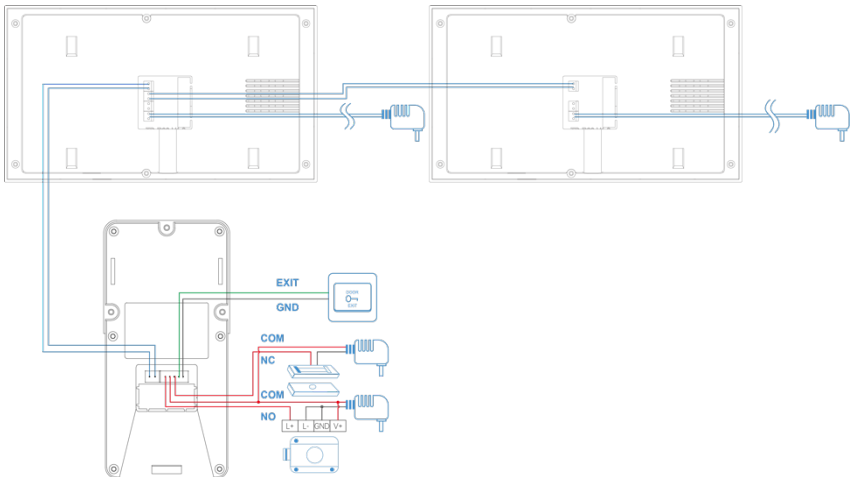
Image 1-4 Standard Connection Diagram 1 Set Outdoor Station to 2 Set Indoor Monitor
