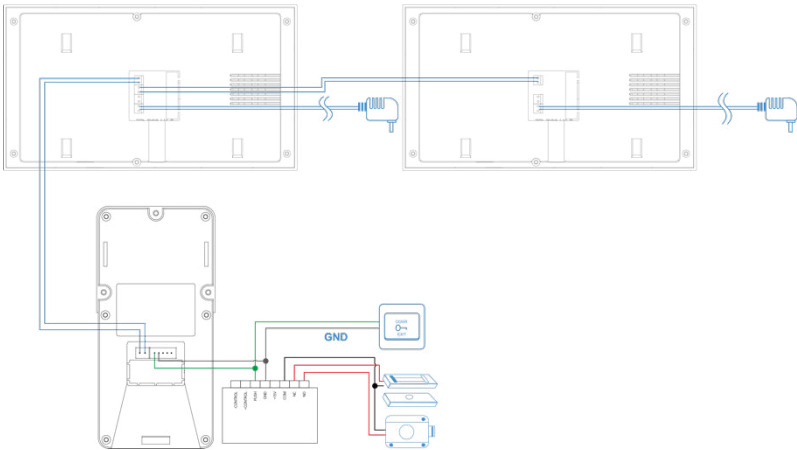
Image 1-7 Access Control Power Connection Diagram 1 Set Outdoor Station to 2 Set Indoor Monitor
