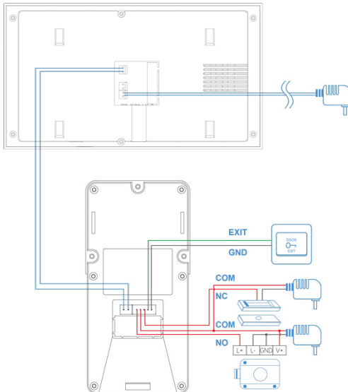
Image 1-3 Standard Connection Diagram 1 Set Outdoor Station to 1 Set Indoor Monitor
