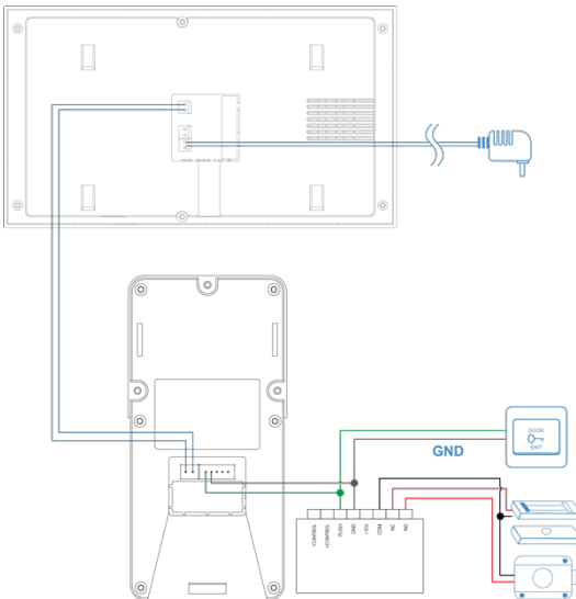
Image 1-6 Access Control Power Connection Diagram 1 Set Outdoor Station to 1 Set Indoor Monitor
