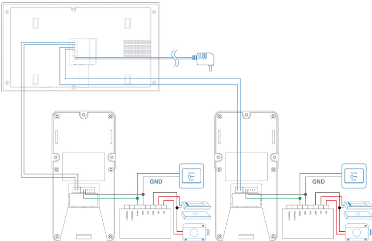
Image 1-8 Access Control Power Connection Diagram 2 Set Outdoor Station to 1 Set Indoor Monitor
