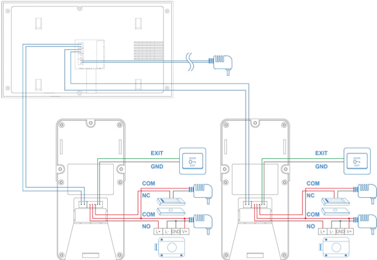
Image 1-5 Standard Connection Diagram 2 Set Outdoor Station to 1 Set Indoor Monitor
