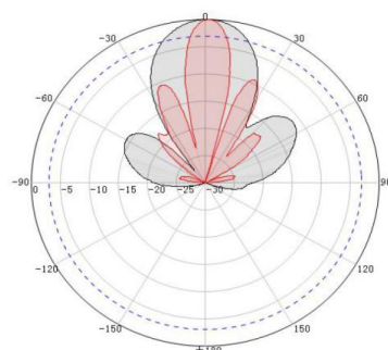
Horizontal polarization
